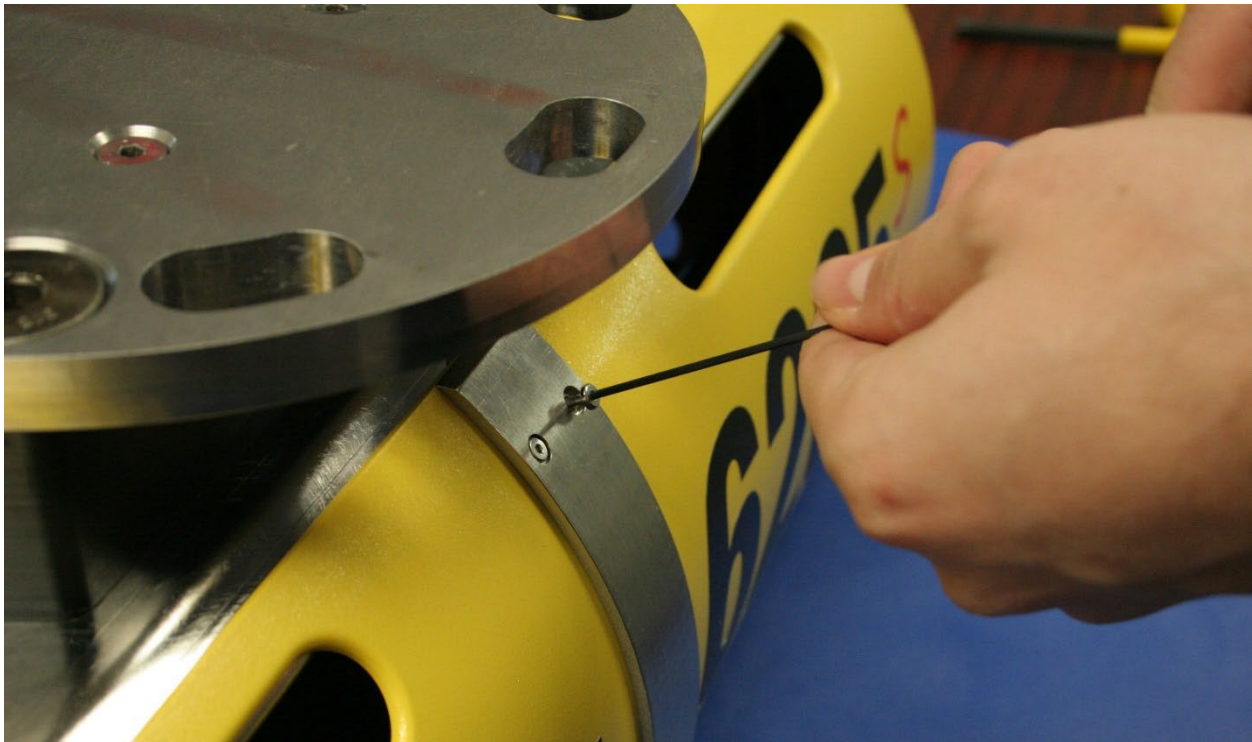
Figure 5-4: Removing the Cap Screws
