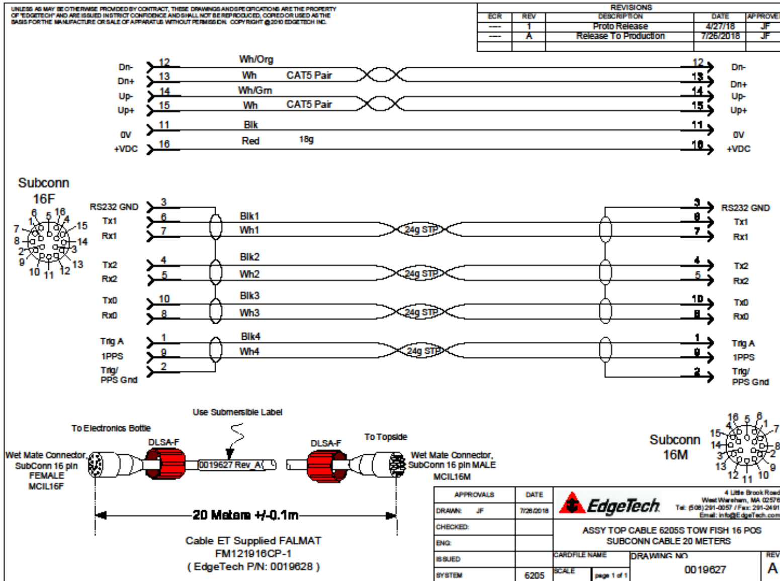
Figure 3-8: 6205s Wiring Diagram – 0019627
