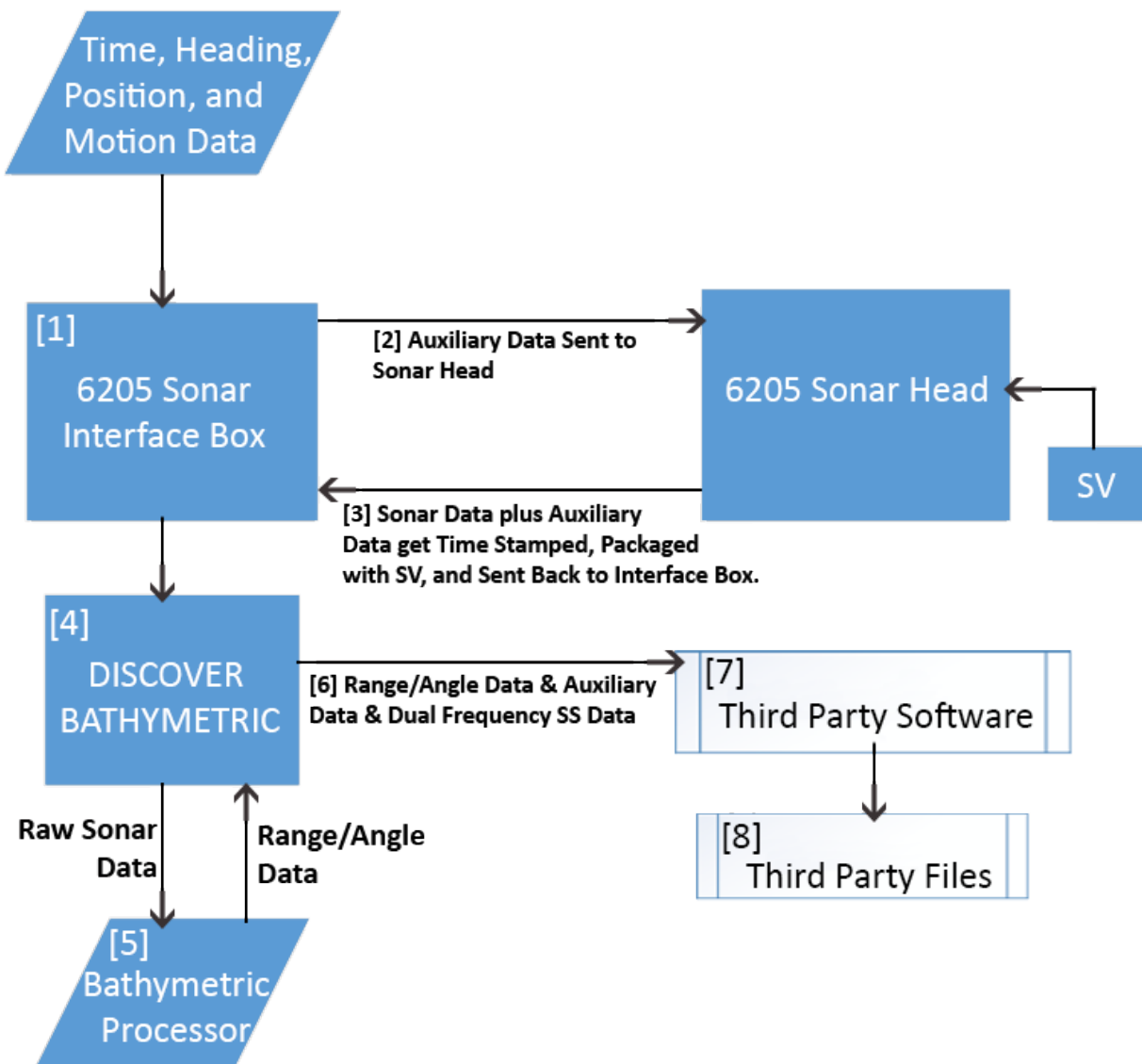
Figure 4-2: Sonar Data Flow
