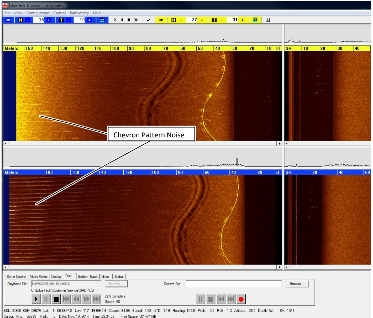
Figure 4-3: Chevron Pattern Noise in a Cropped Portion of Discover Bathymetric
