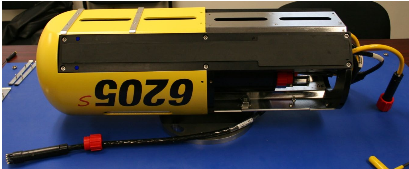
Figure 5-7: Remove the Portion of the Shell 'EdgeTech' and the Logo
