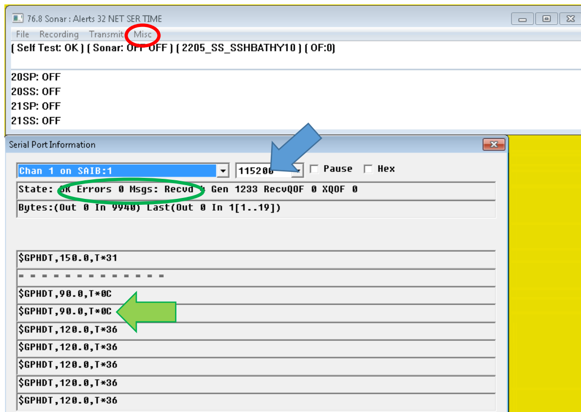
Figure A-7: Checking Serial Port Information
