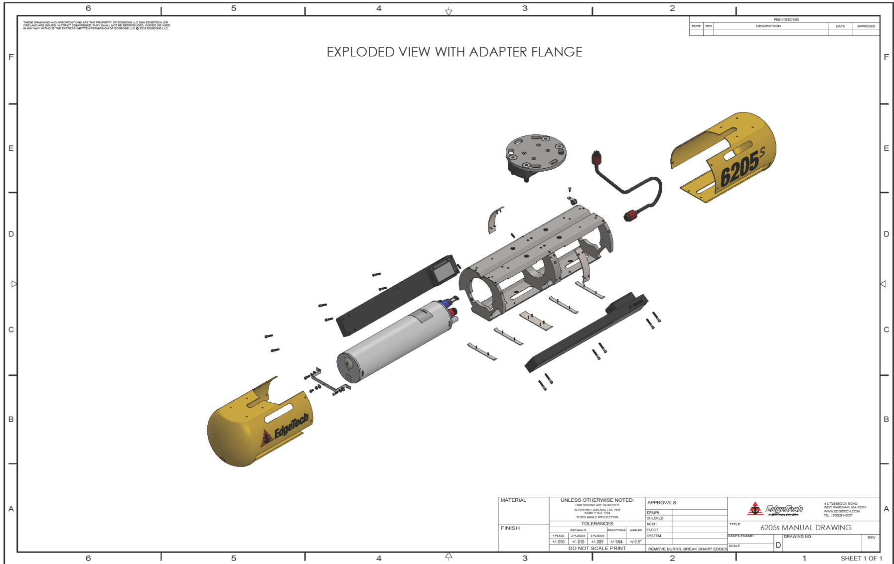
Figure 3-5: 6205s Exploded View with Adaptor Flange
