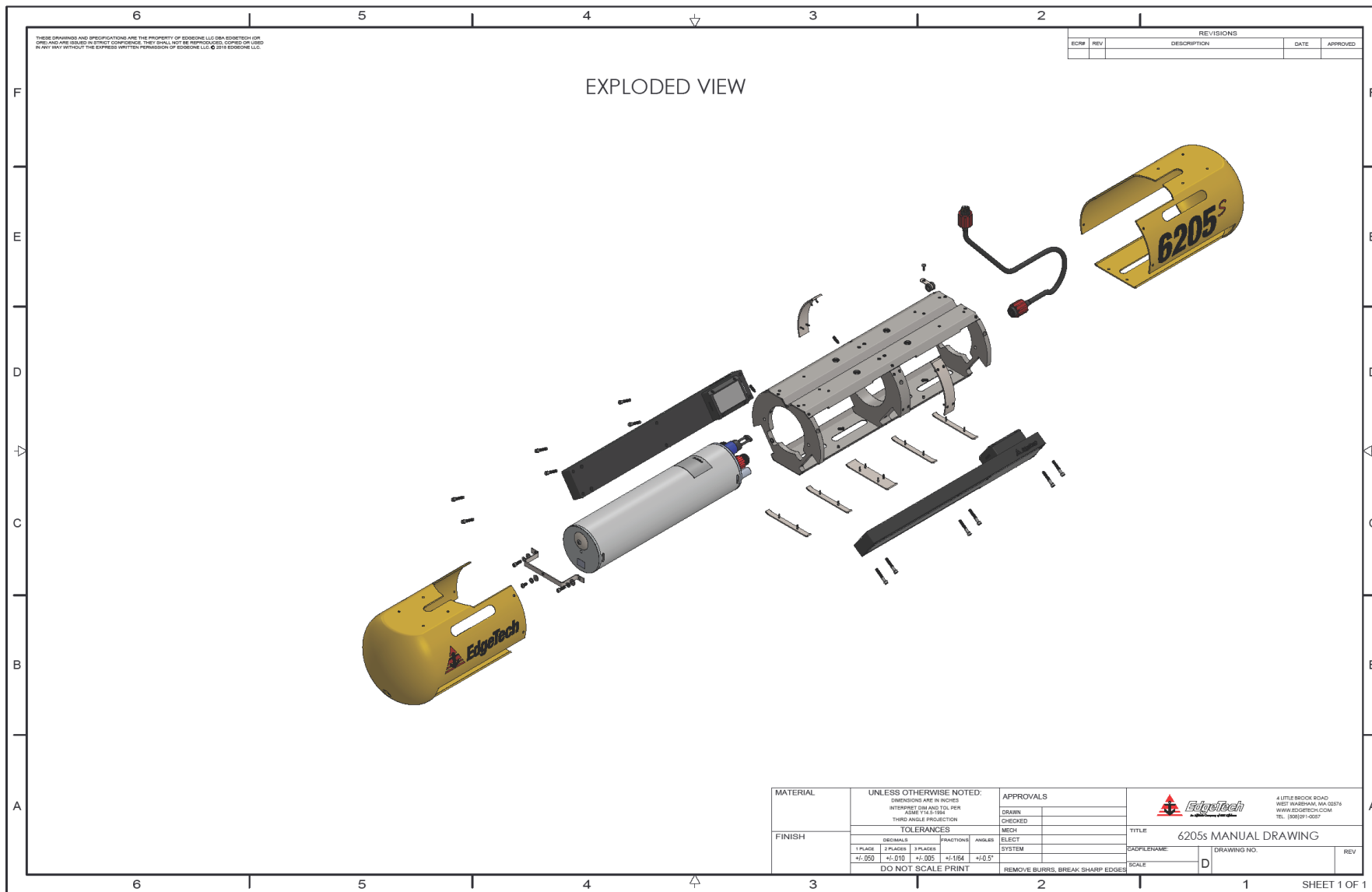
Figure 3-4: 6205s Exploded View
