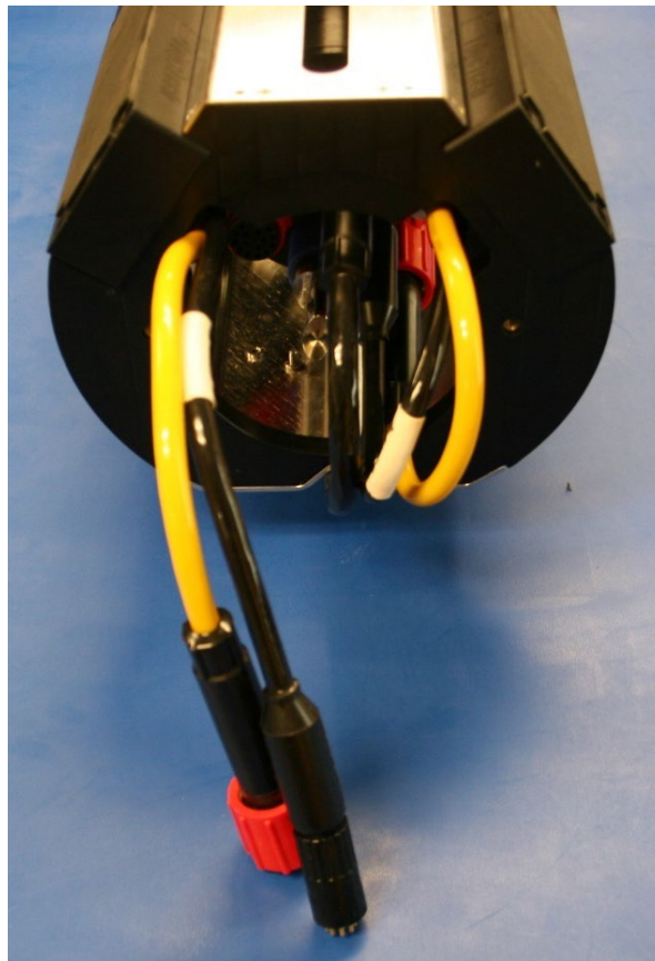
Figure 5-8: The Disconnected Bathymetry and Side Scan Sonar Cables
