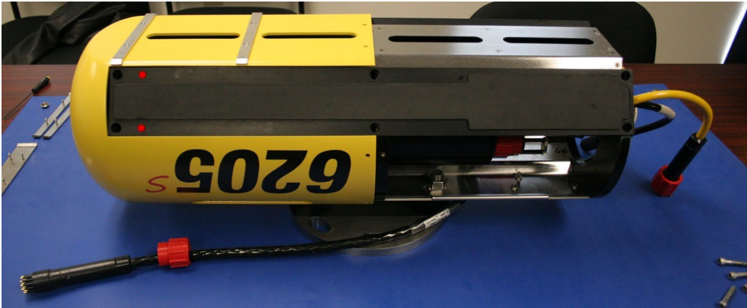
Figure 5-12: Mount the New Transducer
