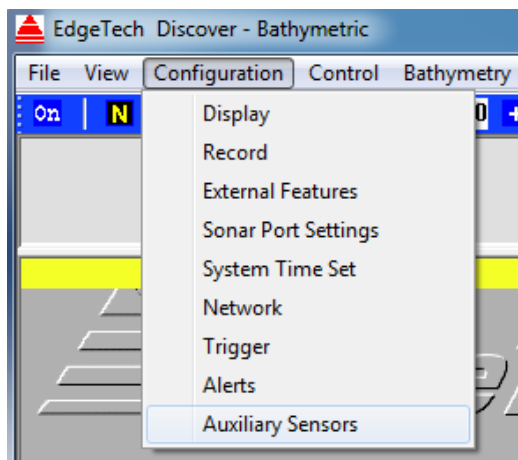
Figure 8-7: Configuration Menu
