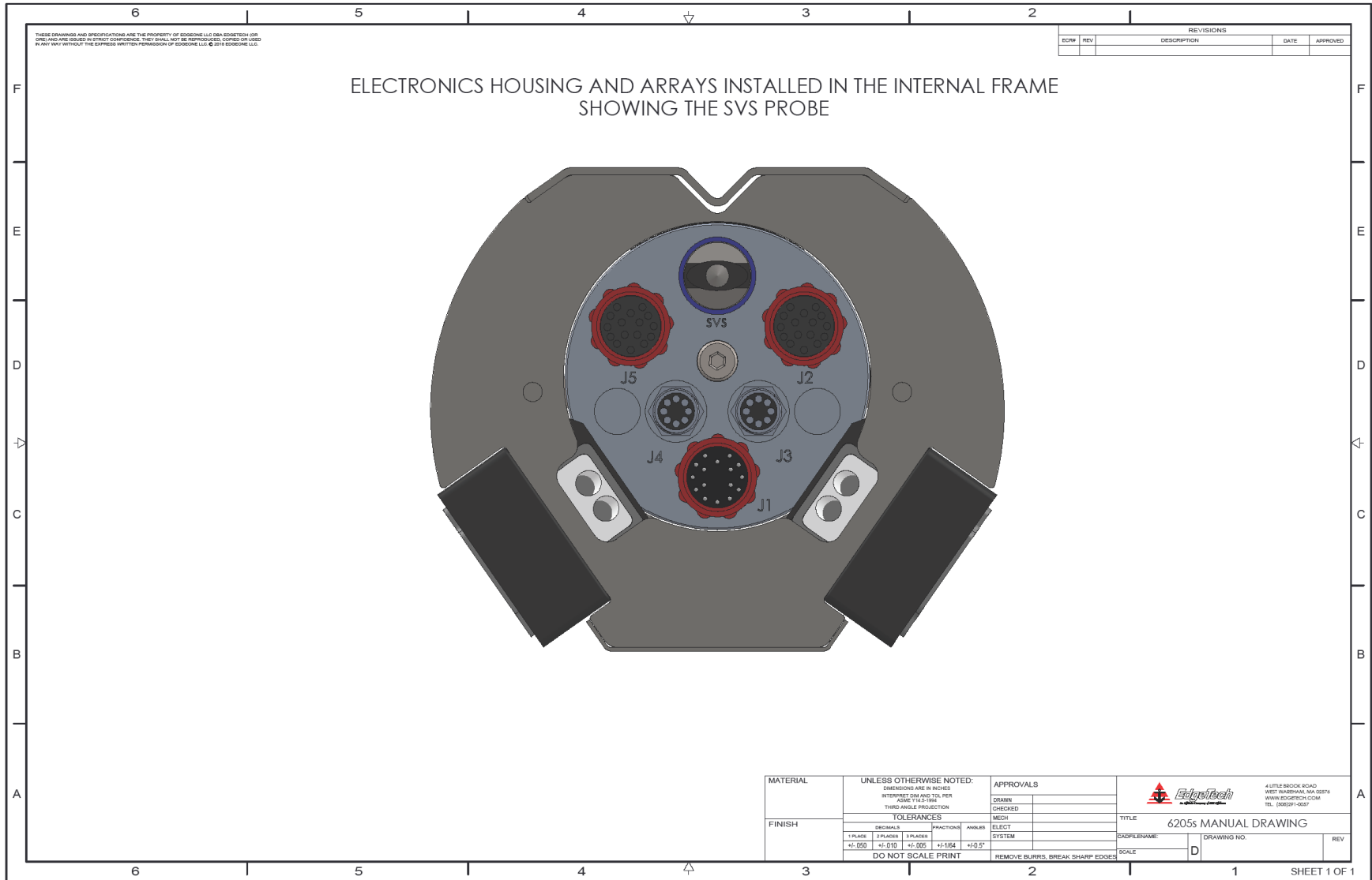
Figure 2-4: 6205s Electronics Housing and Arrays Installed
