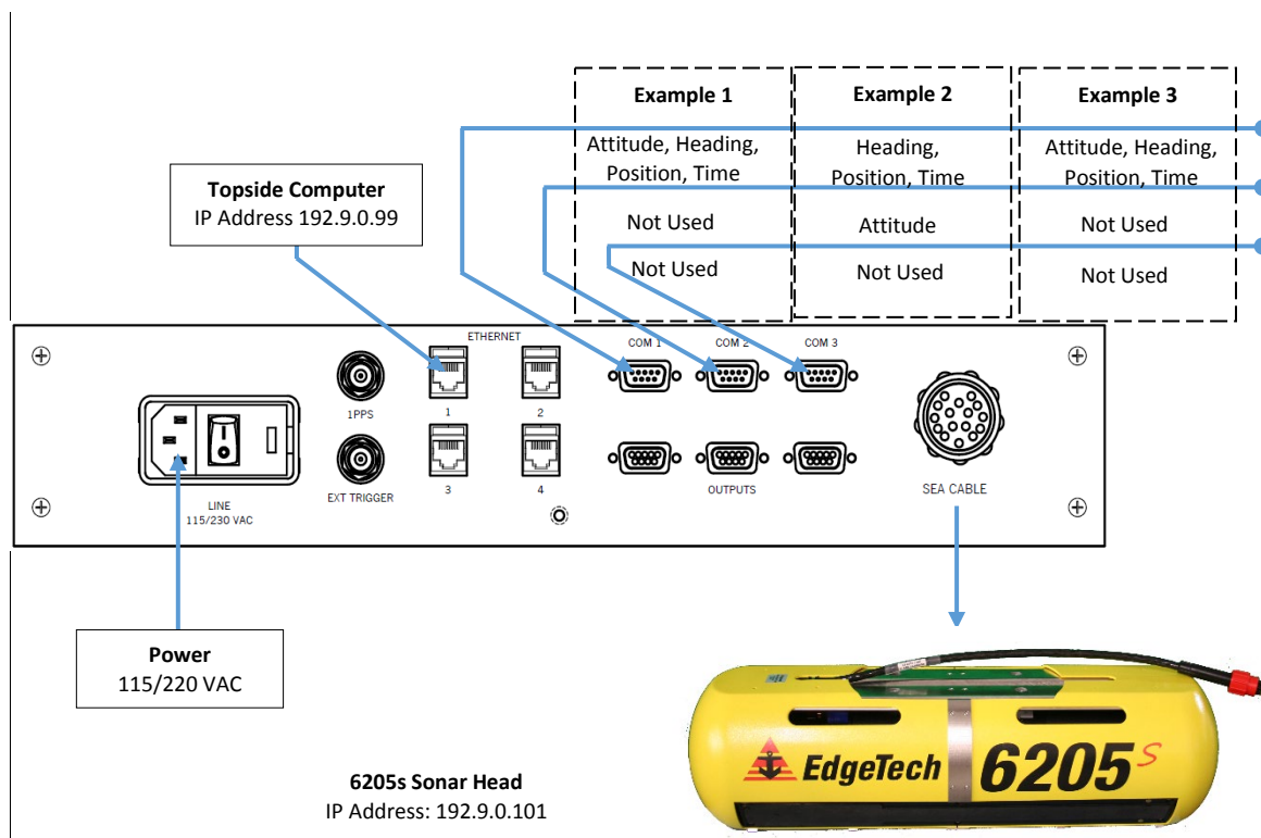
Figure 4-1: 6205s-R Rack Mount Topside Interface Connections
