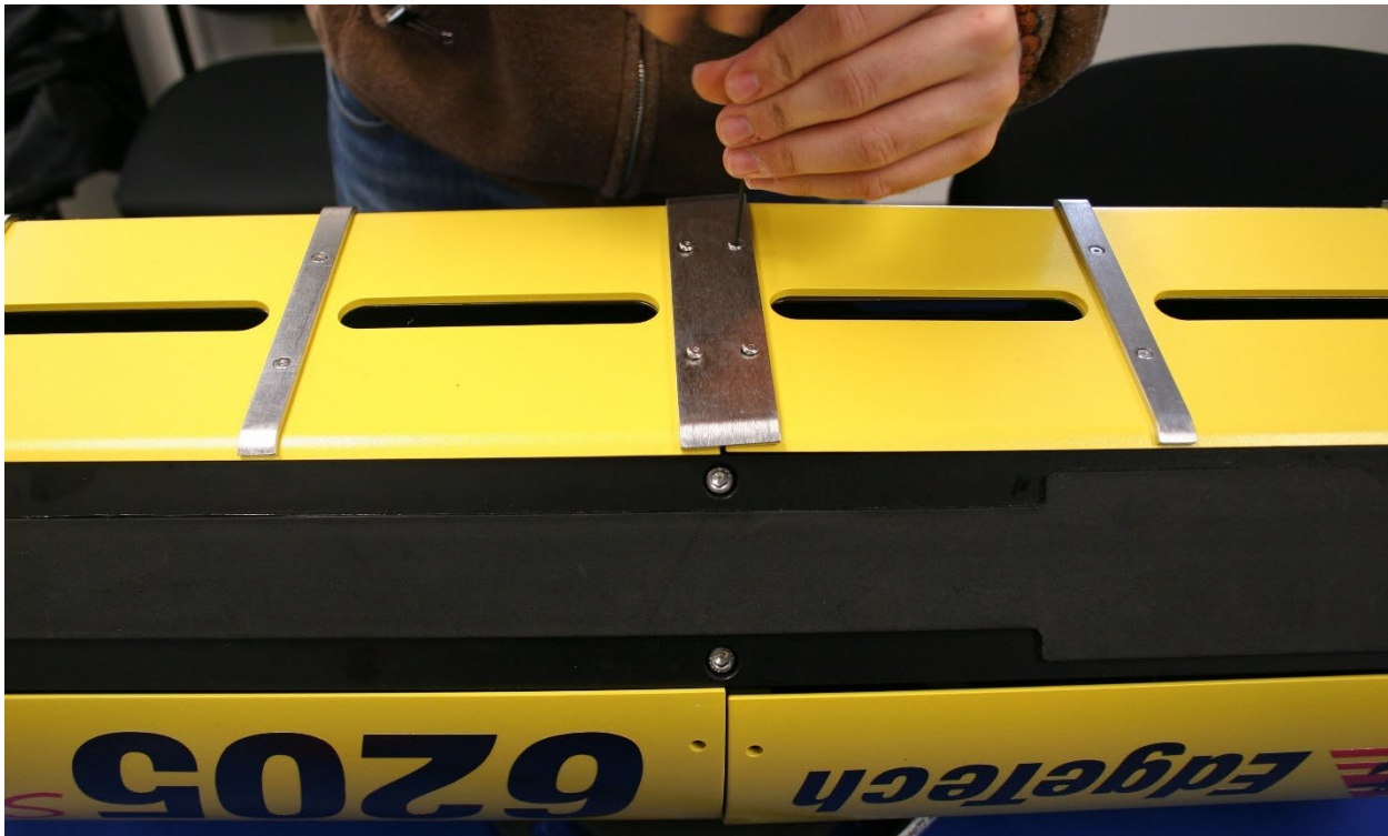
Figure 5-6: Remove the Center Bracket
